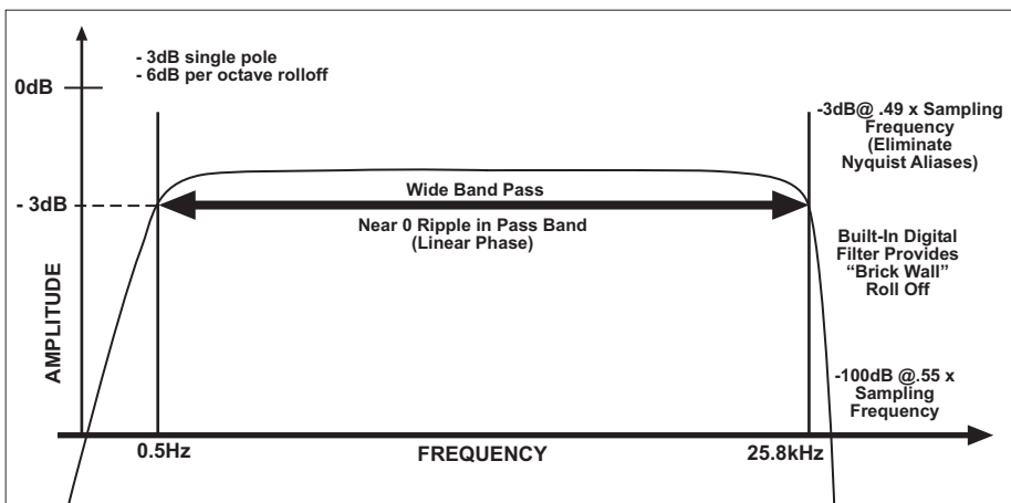
Figure 6. The DT9837A provides software selectable AC and DC coupling. When AC coupling is selected, the modules provide zero ripple in the wide pass band and excellent "brick wall" anti-alias filters eliminating unwanted high frequency interference.
