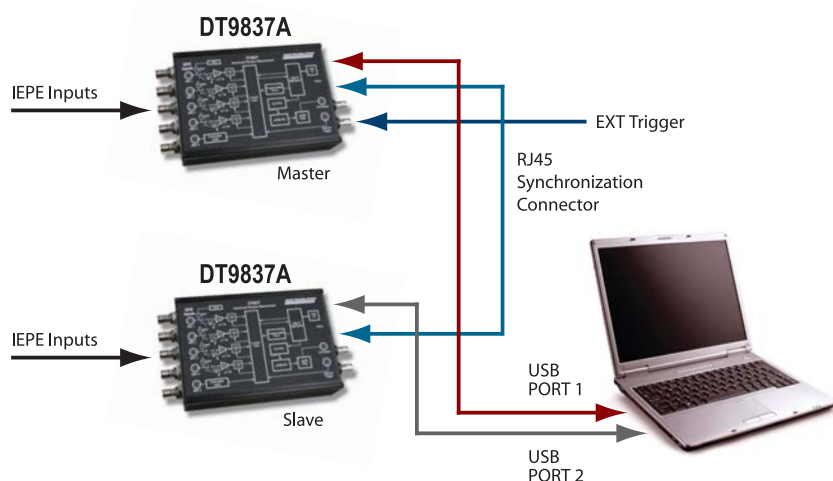
Figure 7. A DT9837A Master/Slave component in Measure Foundry allows two modules to operate in perfect synchronization for 8 IEPE inputs and 2 tachometer inputs.
